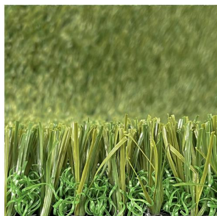
Item: 3AM3024 Pile height: 30mm Gauge: 3/8inch Density: 25200 turfs/sqm
